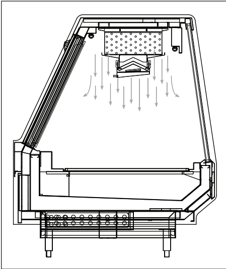
Fig. 11 Airflow pattern
